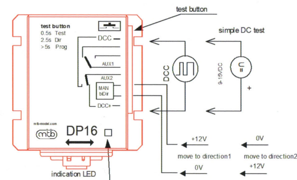
DCC schematic - DP16
